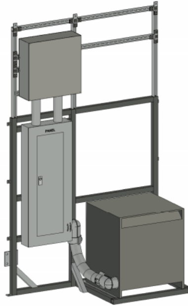
1 75KVA/112KVASUB ASSEMBLY FRAME ISOMETRIC
